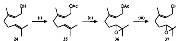
Scheme 7. (i) Ac 2 O, pyridine, 4-DMAP; (ii) mCPBA, NaHCO 3 ; (iii) K 2 CO 3 , 5% aq MeOH.
