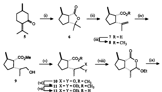
Scheme 1. (i) (a) Br 2 ; (b) NaOMe, MeOH; (c) aq KOH, heat; (ii) Bu t OK, DMF, 140 °C, 3 h; (iii) CH 2 N 2 ; (iv) (a) diisooamylborane; (b) NaOH, H 2 O 2 ; (v) PCC; (vi) HC(OEt) 3 ; TsOH, EtOH; (vii) KOH, aq EtOH; (viii) 100 °C; (ix) 300 °C.
