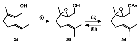
Scheme 6. (i) VO(acac) 3 , t BuOOH, refluxing benzene; (ii) Ac 2 O, pyridine; (iii) K 2 CO 3 , 5% aq MeOH.
