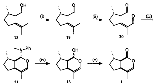
Scheme 2. (i) \text{pyr}_2\text{SO}_3 complex, DMSO, \text{Et}_3\text{N} ; (ii) \text{SeO}_2 , ^t\text{BuOOH} , (iii) \text{MeNHPh} , 4 Å sieves; (iv) \text{TsOH} , \text{THF} : \text{H}_2\text{O} (1:1); (v) \text{AgNO}_3 , Celite, refluxing benzene.
