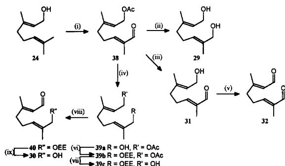
Scheme 8. (i) (a) \text{Ac}_2\text{O} , pyridine, 4-DMAP; (b) \text{SeO}_2 , t\text{-BuOOH} ; (ii) \text{LiAlH}_4 , (iii) \text{K}_2\text{CO}_3 , 5% aq MeOH; (iv) \text{NaBH}_4 ; (v) \text{MnO}_2 (active); (vi) ethyl vinyl ether, TsOH; (vii) \text{K}_2\text{CO}_3 , 5% aq MeOH; (viii) \text{MnO}_2 (active); (ix) MeOH, TsOH.
